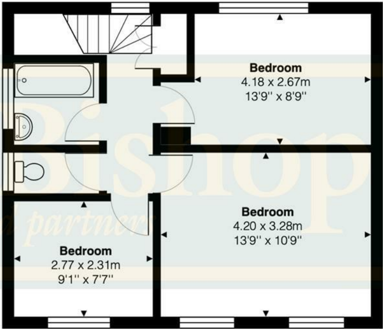
First Floor Area: 43.2 m 2 ... 465 ft 2
